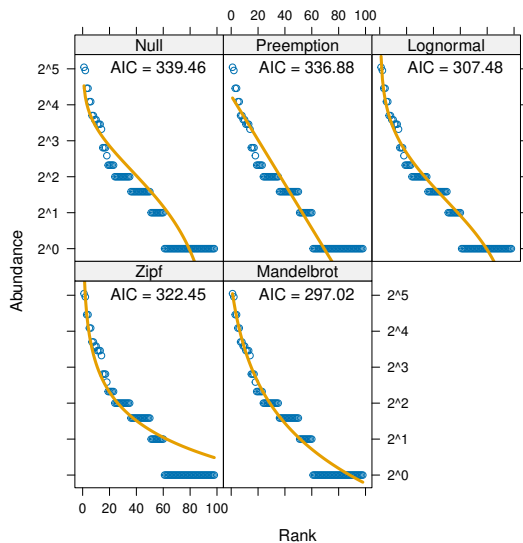
Figure 4: Ranked abundance distribution models for a random plot (no. 14). The best model has the lowest AIC.
