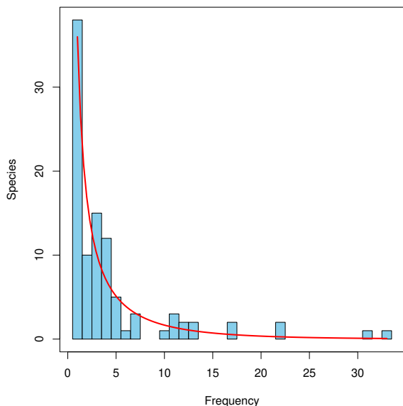
Figure 3: Fisher’s log-series fitted to one randomly selected site (14).
